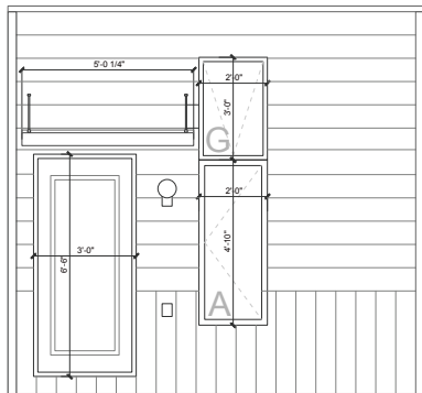
FRONT EXTERIOR ELEVATION
