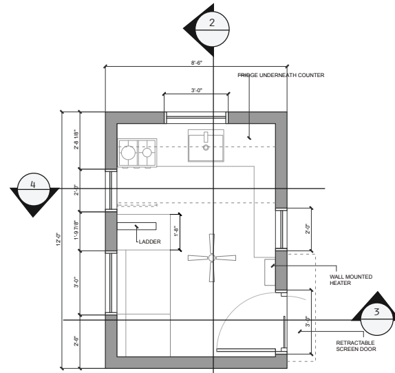
FLOORPLAN - MAIN LEVEL
