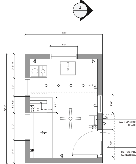
ELECTRICAL PLAN - MAIN LEVEL
