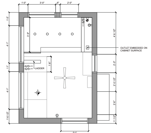
ELECTRICAL PLAN - LOFT LEVEL
