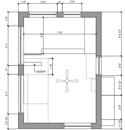
FLOOR PLAN - LOFT LEVEL
