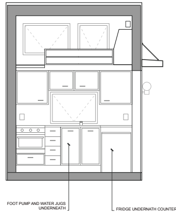
SECTION 2 INTERIOR ELEVATION SHOWING WINDOWS, BUILT IN COUCH, KITCHEN AREA AND LOFTS
