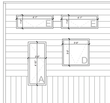
BACK EXTERIOR ELEVATION
